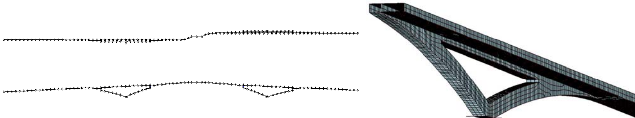
Fig. 3 - Plan and side view of the beam finite element mesh. Detail of shell finite element model
