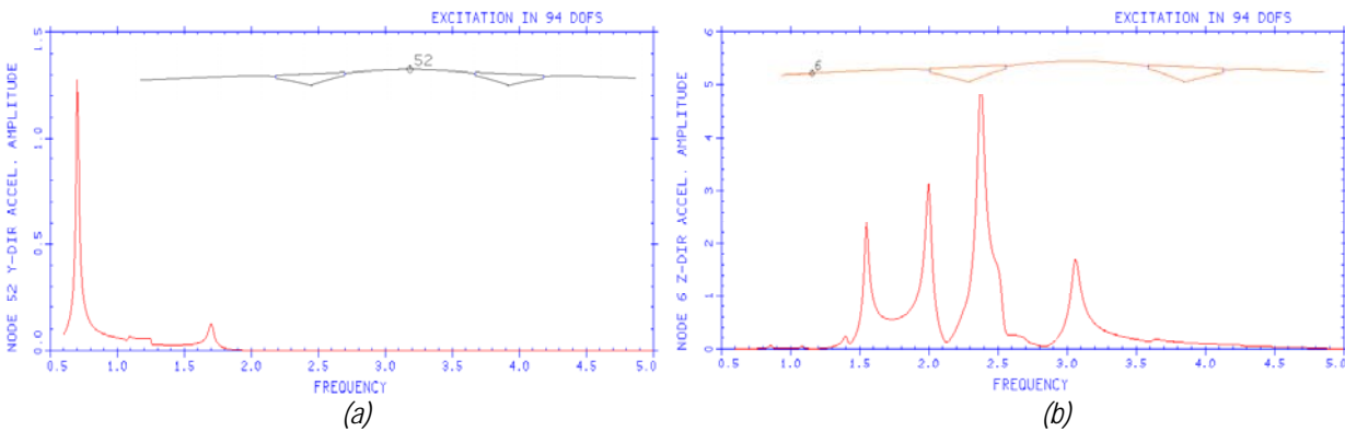
Fig. 6 - Spectral acceleration associated uniformly distributed pedestrian load (1person/m 2 ): (a) lateral acceleration at mid-span; (b) vertical acceleration at mid-point of transition span (m/s 2 )
