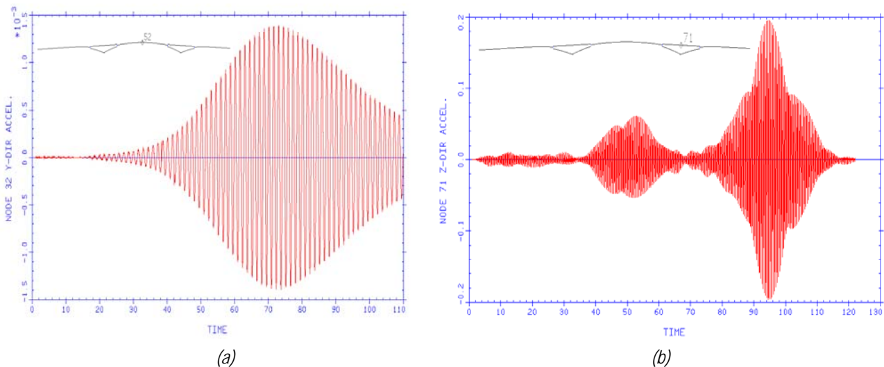
Fig. 5 - Response history associated with single pedestrian propagation: (a) lateral acceleration at mid-span for f_p=0.704\text{Hz} ; (b) vertical acceleration at mid-point of tie for f_p=2.522\text{Hz} ( \text{m/s}^2 )
