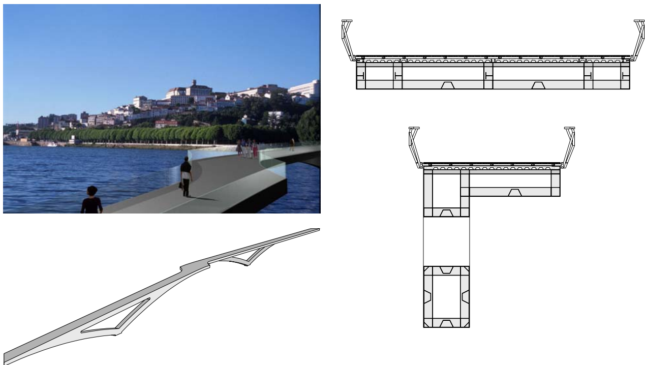
Fig. 2 - Perspectives of the footbridge. Cross-sections at mid-span and at in the proximity of the arch springs
